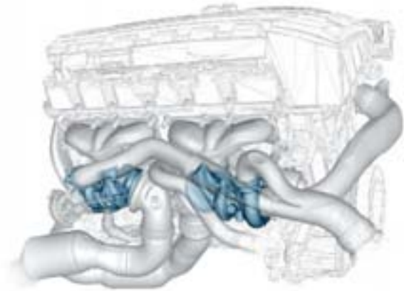
Fast buildup of pressure: the two parallel turbochargers (shown in blue) make a key contribution to the outstanding responsiveness of the 135i s inline six-cylinder engine.
