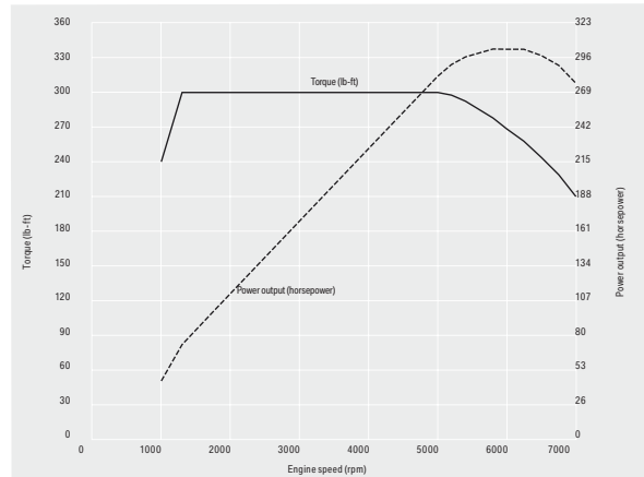
Portrait of an engineering masterpiece: the 135i twin-turbo engine produces 300 hp at 5800 rpm, and quickly develops 300 lb-ft of torque at 1400 rpm, which continues without fading through to the 5000-rpm range. With such a broad range of powerful torque, you can enjoy smooth, robust acceleration in any gear, at any speed.
