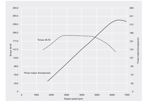
Portrait of an engineering masterpiece: the 3.0-liter engine pours on the power and quickly develops maximum torque, which continues without fading over a large rpm range – so you enjoy smooth, powerful acceleration at virtually any legal speed.
