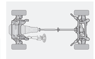
Lightweight construction is used throughout the 3 Series Sports Wagon. In both the 328i and 328i xDrive, the five-link rear suspension includes cast-aluminum upper transverse arms. In the front section of the 328i, aluminum is used extensively for suspension components, including forged-aluminum lower arms and the steering knuckle, as well as the subframe and the steering rack.
