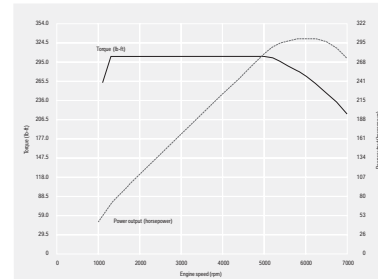
Portrait of a masterpiece: the 535i xDrive's twin-turbo engine produces 300 horsepower at 5800 rpm, and quickly develops 300 lb-ft of torque at 1400 rpm, which continues without fading through to the 5000 rpm range. With such a broad range of powerful torque, you can enjoy smooth, robust acceleration in any gear, at any speed.
