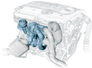
Fast buildup of pressure: the two parallel turbochargers (shown in blue) make a key contribution to the outstanding responsiveness of the 535i xDrive's inline six-cylinder engine.
