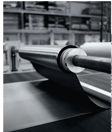
Carbon sheets are delivered on rollers and layered one atop the other (right). Robots transport the pre-formed roof (far right) to the large press for injection of the resin (below).
