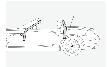
■ Z4 Roadster rollover protection consists of two steel roll bars behind the headrests; they are connected with a highly stable chassis crossbeam. The system is completed by a bar of high-strength tubular steel integrated into the windshield frame for maximum safety.
