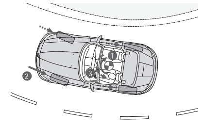
■ Cornering Brake Control (CBC) increases vehicle stability by proportioning the braking force while turning. When you brake in a turn, the pressure comes off the rear wheels, which (1) causes the vehicle to swerve inward (oversteer). Cornering Brake Control counteracts this action by asymmetrically adjusting brake pressure (2), creating stabilizing counter-torque (3) independently of the ABS system.
