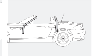
Z4 Roadster Rollover Protection System consists of two steel roll bars behind the headrests; they are connected with a highly stable chassis crossbeam. The system is completed by a bar of high-strength tubular steel integrated into the windshield frame for maximum safety.
