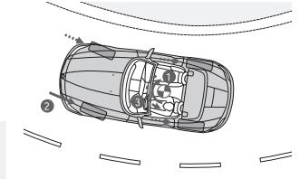
Cornering Brake Control (CBC) increases vehicle stability by proportioning the braking force while turning. When you brake in a turn, the pressure comes off the rear wheels, which (1) causes the vehicle to swerve inward (oversteer). Cornering Brake Control counteracts this action by asymmetrically adjusting brake pressure (2), creating stabilizing counter-torque (3) independently of the ABS system.
