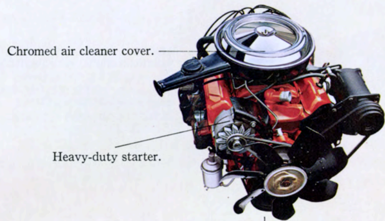
200-hp Turbo-Fire 350 V8. Or available 240-hp Turbo-Jet 396 V8.
