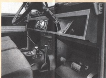
The driving compartment, showing arrangement of instruments and controls.
