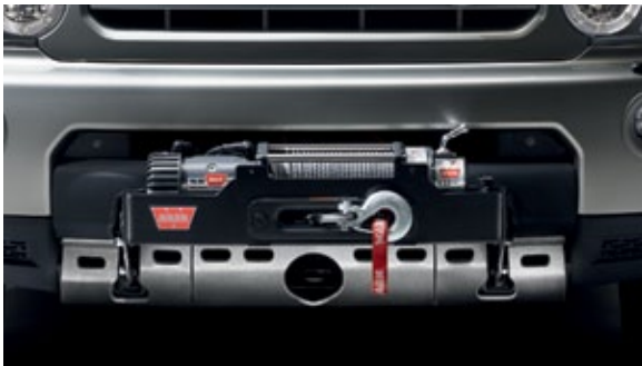
Electric Winch† VUB501471 9,500lbs/4,300kg maximum load capacity. Includes cover for protection when not in use. Plug-in remote control allows safe operation from up to 11.8ft/3.6 meters. Compatible with Protection Bar (VPLAP0022).
