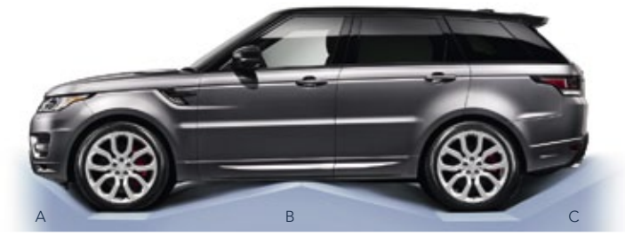
Obstacle Clearance Off-road height 10.9 inches Standard ride height 8.4 inches
