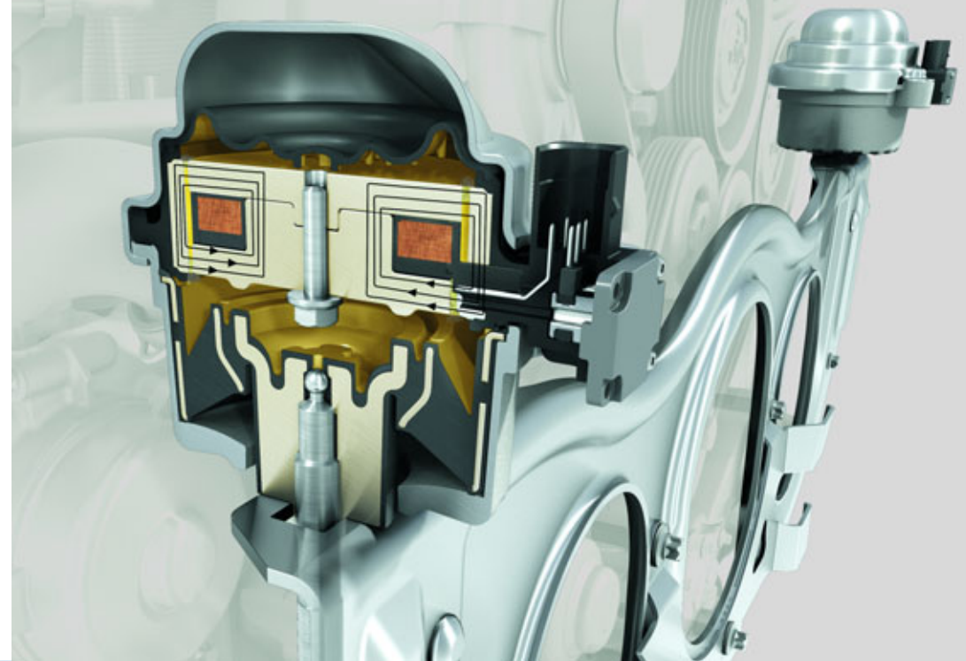
Dynamic engine mount system
