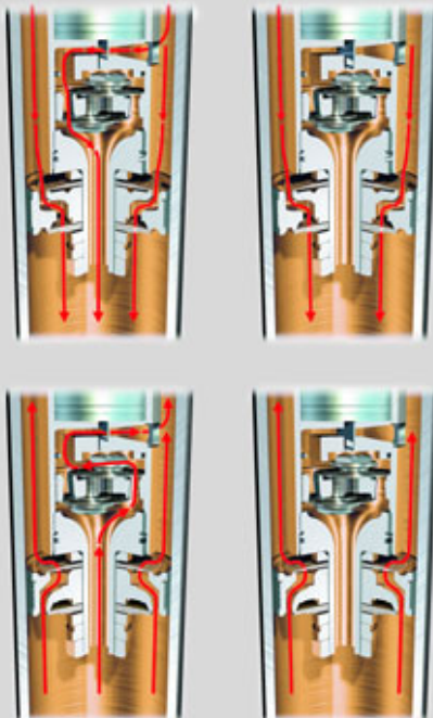
Left: Rebound in 'Normal' mode – damper piston and bypass valve
