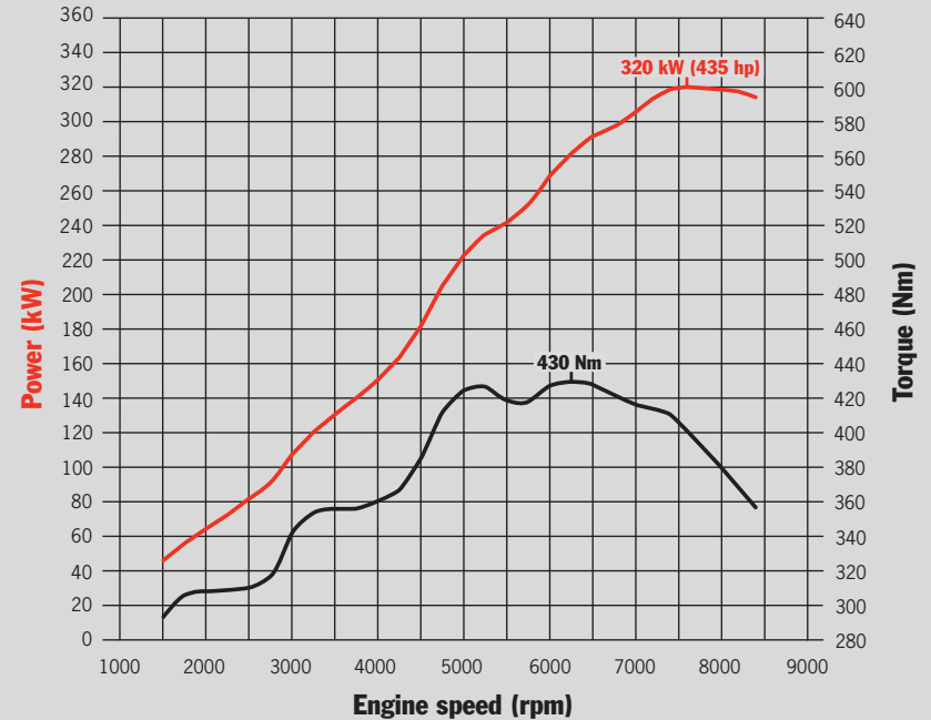
911 GT3: 430 Nm at 6,250 rpm, 320 kW (435 hp) at 7,600 rpm
