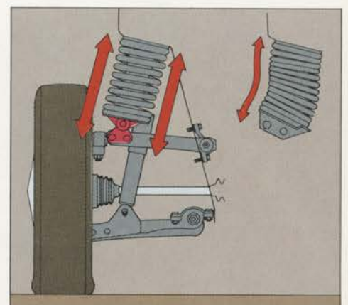
Pivoted front springs working at full capacity without any bending tendencies.
