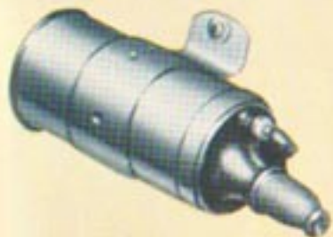
Ignition coil inverted on eight, horizontal on six . . . reduces chance of moisture affecting electrical system. Shorter high-tension lead improves spark, reduces radio interference.
