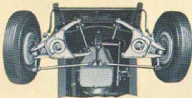
Center-Point Steering acts equally on either wheel; most accurately designed and easy to handle steering system known. Formerly found only in the most costly cars.
